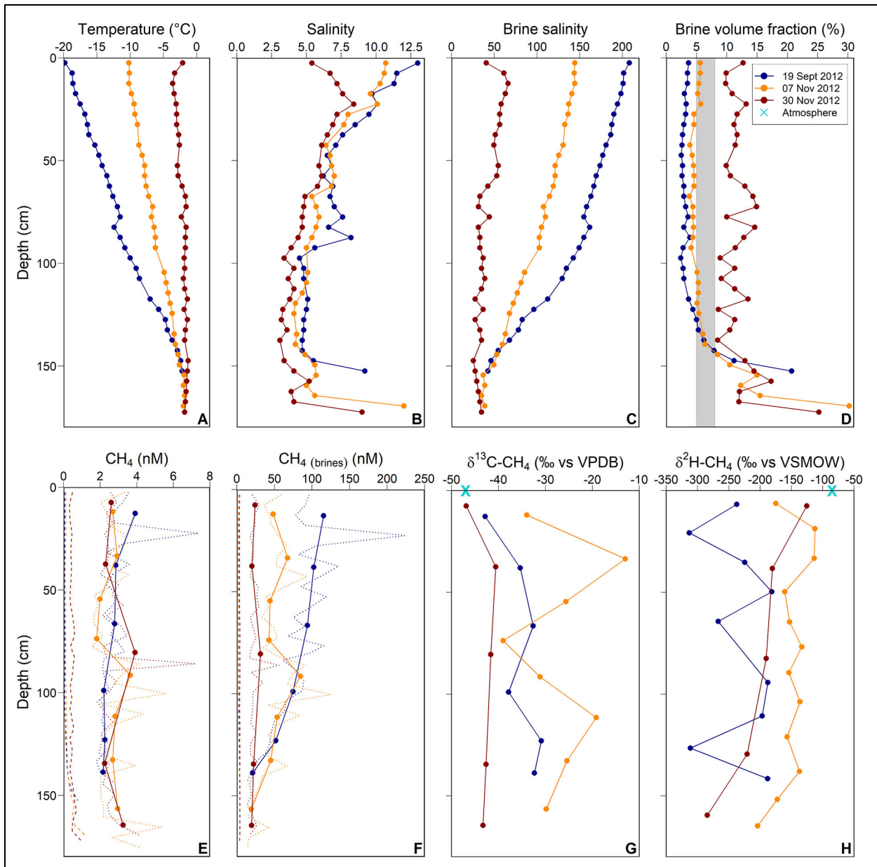
Figure 4. Summary of Cape Evans (Antarctic) sea-ice data. Upper panels show Cape Evans sea-ice physical properties, adapted from Carnat et al. (2014): (A) temperature (°C), (B) salinity, (C) brine salinity, and (D) brine volume fraction (%), in cores collected on September 19 (blue), November 7 (orange), and November 30 (red). The shaded gray area in (D) encompasses the permeability threshold for brines (5%) defined in (Golden et al., 1998) and for gases (7%–8%) defined in Zhou et al. (2013). Lower panels show vertical profiles of (E) CH 4 concentrations (nM) in bulk ice (for readability, we did not add error bars that span \pm 1.1 nM), (F) CH 4 concentrations (nM) in brines, (G) \delta^{13}\text{C}\text{-CH}_4 (‰ vs. Vienna Pee Dee Belemnite) with a standard deviation of \pm 0.4 ‰, and (H) \delta^2\text{H}\text{-CH}_4 (‰ vs. Vienna Standard Mean Ocean Water) with a standard deviation of < 5 ‰, in sea cores from Cape Evans, collected on September 19 (blue), November 7 (orange), and November 30 (red). The dashed lines in (E) represent the calculated equilibrium solubility. The dotted lines in (E) and (F) represent the concentrations measured at a 5-cm resolution and averaged to meet the isotopic resolution (solid lines). The light blue cross represents the isotopic composition of the atmosphere. DOI: https://doi.org/10.1525/elementa.2020.00167.f4
